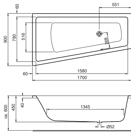
Eckwanne links 1700 x 900/600 x 450 mm Corner bathtub, left 1700 x 900/600 x 450 mm
