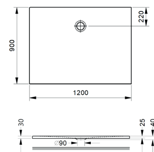
Duschebene Quadrat Shower tray, square 1200 x 900 x 18 mm
