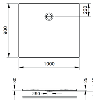
Duschebene Quadrat Shower tray, square 1000 x 900 x 18 mm
