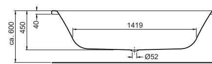
Rechteckwanne 1900 x 900 x 450 mm Rectangular bathtub 1900 x 900 x 450 mm
