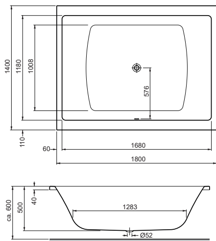
Rechteckwanne 1800 x 1400 x 500 mm Rectangular bathtub 1800 x 1400 x 500 mm
