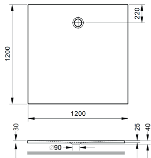
Duschebene Quadrat 1200 x 1200 x 18 mm Shower tray, square 1200 x 1200 x 18 mm
