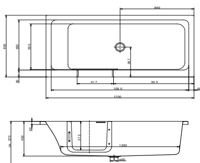
Duschbadewanne, Tür links Rectangular bathtub with shower area, door on left side 1700 x 800 x 570 mm
