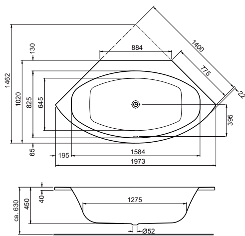
Vario - Eckwanne NOVA 1400 x 1400 x 450 mm Vario - corner bathtub NOVA 1400 x 1400 x 450 mm
