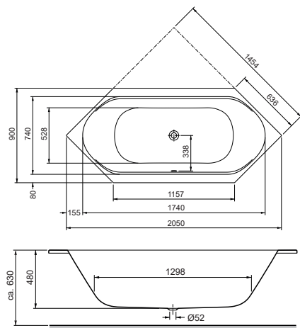
Sechseckwanne 1700 x 800 x 480 mm Six-sided bathtub 1700 x 800 x 480 mm
