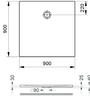
Duschebene Quadrat 900 x 900 x 18 mm Shower tray, square 900 x 900 x 18 mm
