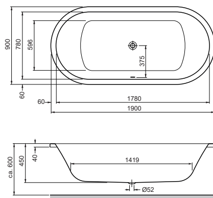
Ovalwanne 1900 x 900 x 450 mm Oval bathtub 1900 x 900 x 450 mm
