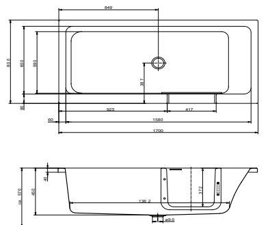
Duschbadewanne, Tür rechts Rectangular bathtub with shower area, door on right side 1700 x 800 x 570 mm
