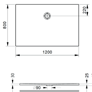
Duschebene Quadrat Shower tray, square 1200 x 800 x 18 mm
