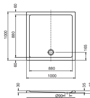
Duschwanne Quadrat Shower tray, square 1000 x 1000 x 35 mm
