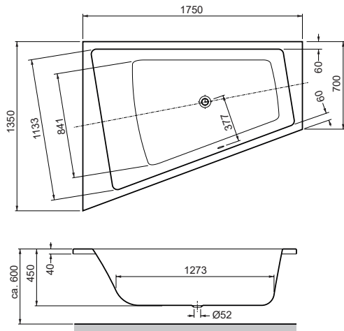
Eckwanne links 1750 x 1350/700 x 450 mm Corner bathtub, left 1750 x 1350/700 x 450 mm
