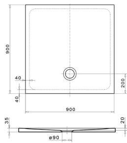
Duschwanne Quadrat shower tray, square 900 x 900 x 35 mm
