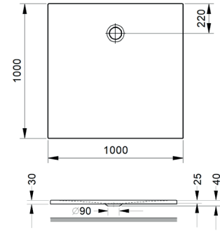
Duschebene Quadrat 1000 x 1000 x 18 mm Shower tray, square 1000 x 1000 x 18 mm
