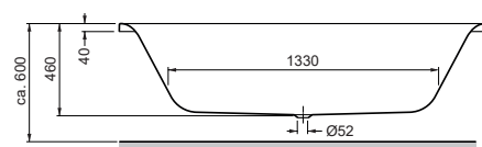
Ovalwanne Mittelablauf 1850 x 900 x 460 mm Oval bathtub, central drain 1850 x 900 x 460 mm
