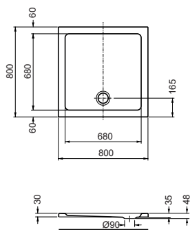
Duschwanne Quadrat Shower tray, square 800 x 800 x 35 mm
