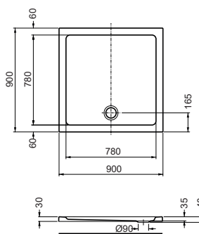
Duschwanne Quadrat Shower tray, square 900 x 900 x 35 mm
