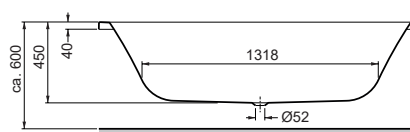
Rechteckwanne 1800 x 800 x 450 mm Rectangular bathtub 1800 x 800 x 450 mm
