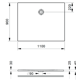
Duschebene Quadrat Shower tray, square 1100 x 900 x 18 mm
