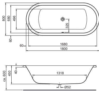
Ovalwanne 1800 x 800 x 450 mm Oval bathtub 1800 x 800 x 450 mm
