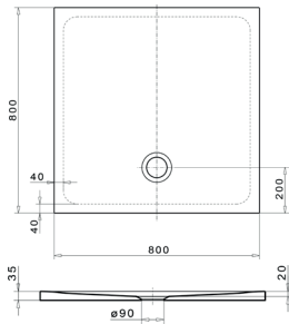
Duschwanne Quadrat shower tray, square 800 x 800 x 35 mm
